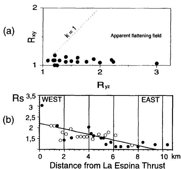
Fig. 6. (a) Flinn plot showing that all the samples analyzed fall into the apparent flattening field. (b) Plot of R_s values vs distance from La Espina Thrust. Data have been projected along the strike of the structures into the vertical surface of the cross-section in Fig. 3. Best fit line calculated from the 3D ellipsoids (black dots). 2D ellipsoids are represented by white dots and are less indicative as they are further away from the section trace and, therefore, projection into A-A' is more speculative.
