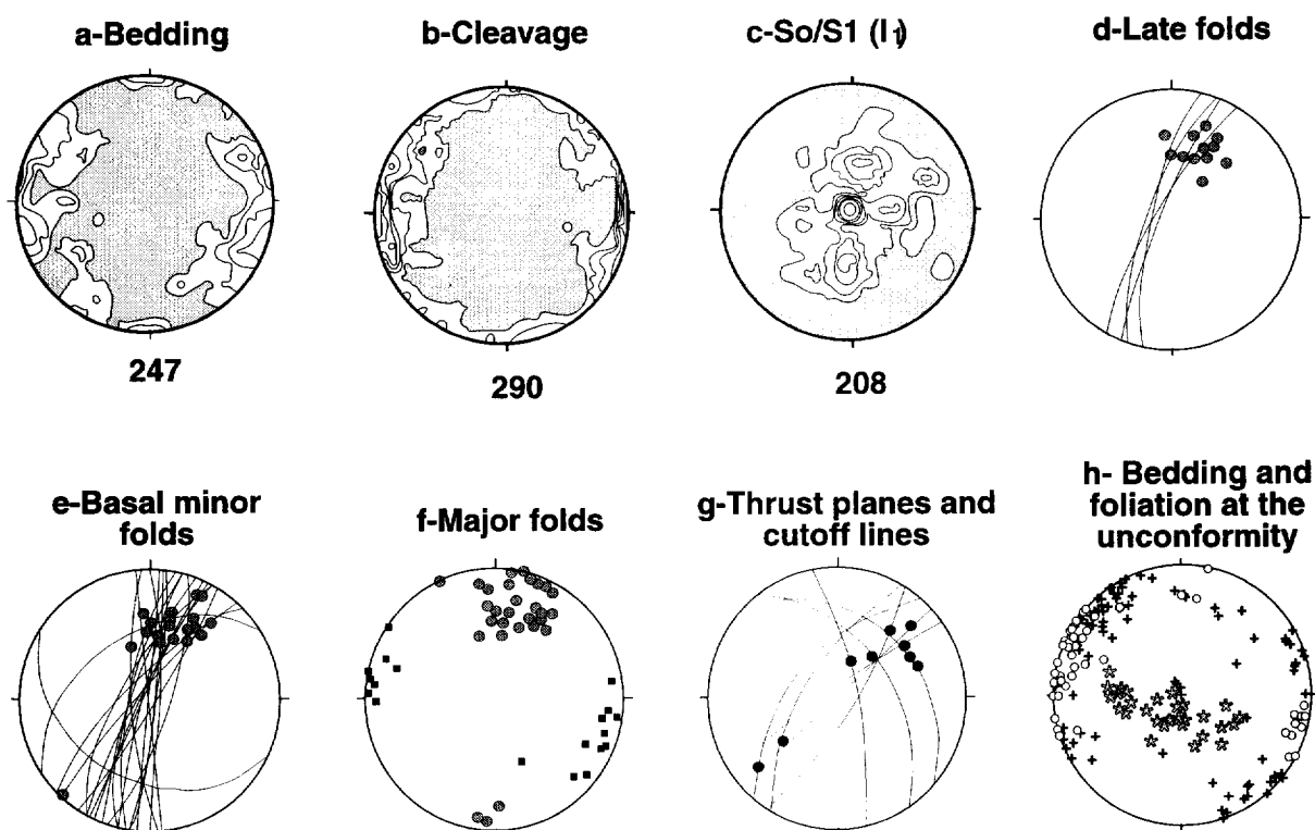
Fig. 4. Orientation of the main structural features observed in the Narcea Slates (a–d) and the Herreria Quartzites (e–g). (a) Density contours of poles to bedding planes. (b) Density contours of poles to cleavage planes. (c) Density contours of S_0/S_1 intersection lineation ( l_1 ). Schmidt projection, lower hemisphere, 2% contours for 1% area. Number of measurements indicated. Grey pattern < 2%. (d) Axes and axial planes of folds affecting the Narcea slates foliation. These folds are related to the late out-of-sequence thrusting. (e) Folds related to minor thrusts, great circles are axial planes and dots are fold axes. (f) Major folds in the Herreria Quartzite, dots are fold axes and squares are poles to axial planes. (g) Thrust planes and cutoff lines developed in the basal beds of the Herreria Quartzites, showing both frontal and lateral features. (h) Bedding of the Narcea Slates (crosses), the Herreria Quartzites (stars) and cleavage in the Narcea Slates (dots) close to the unconformity–decollement plane. Note the vertical attitude of bedding, cleavage and intersection lineation in the Narcea Slates.
