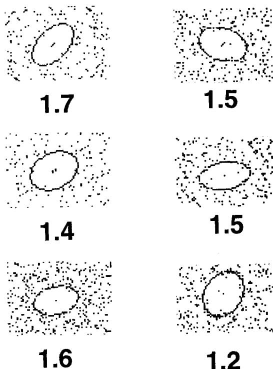
Fig. 5. Some examples of Fry analysis samples used in this work with the R_s values obtained.
